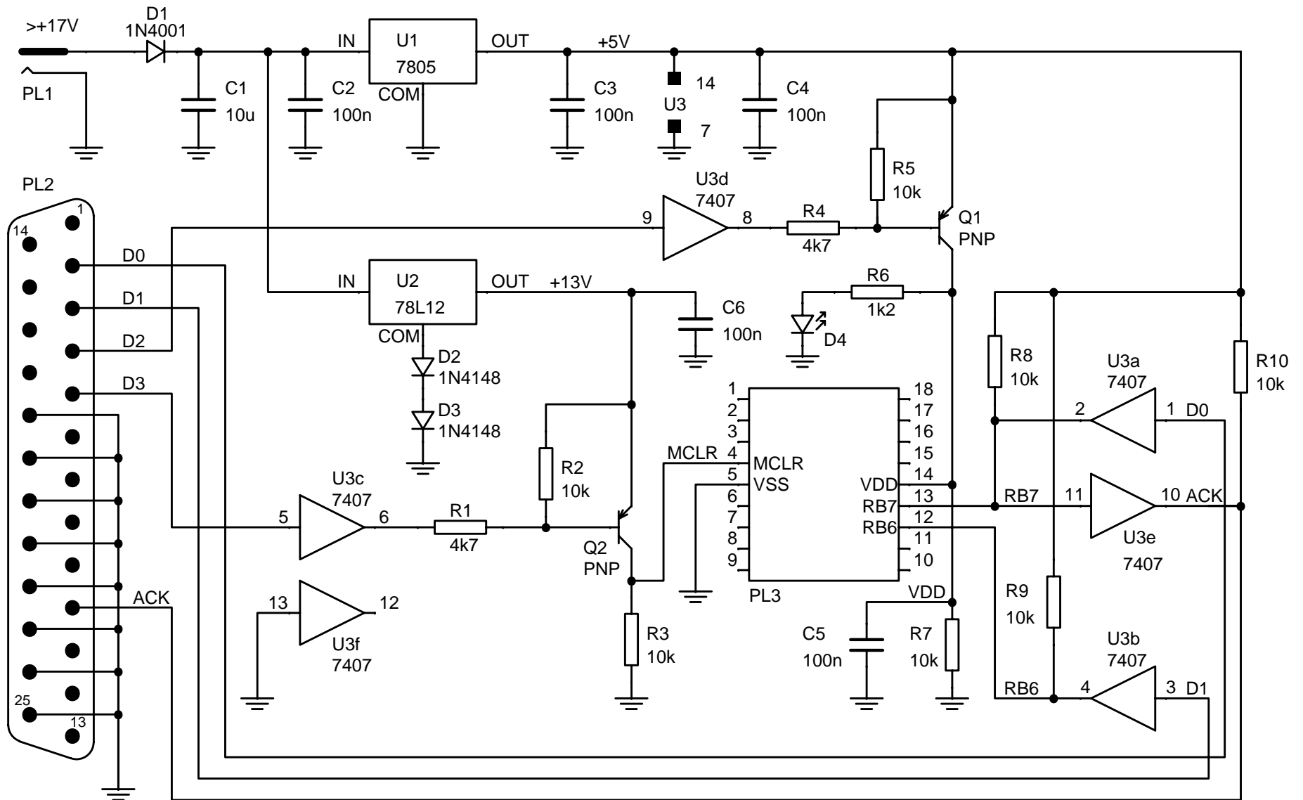
'Classic' PIC16F84 Programmer
